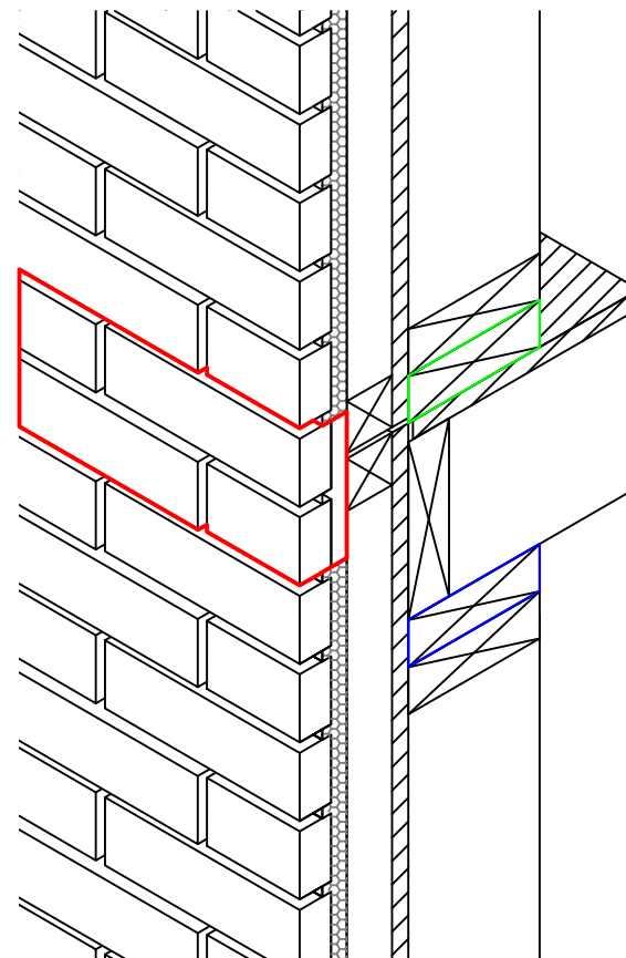
Two courses site filled for panel fixing
