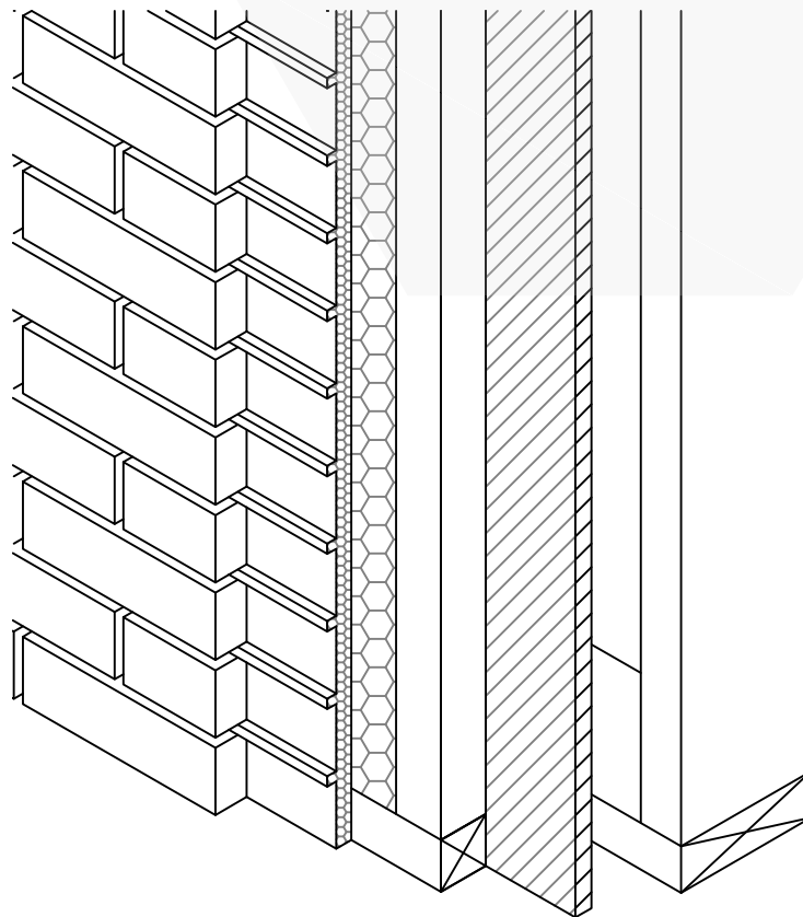
Typical external wall: 0.14 W/m 2 k
