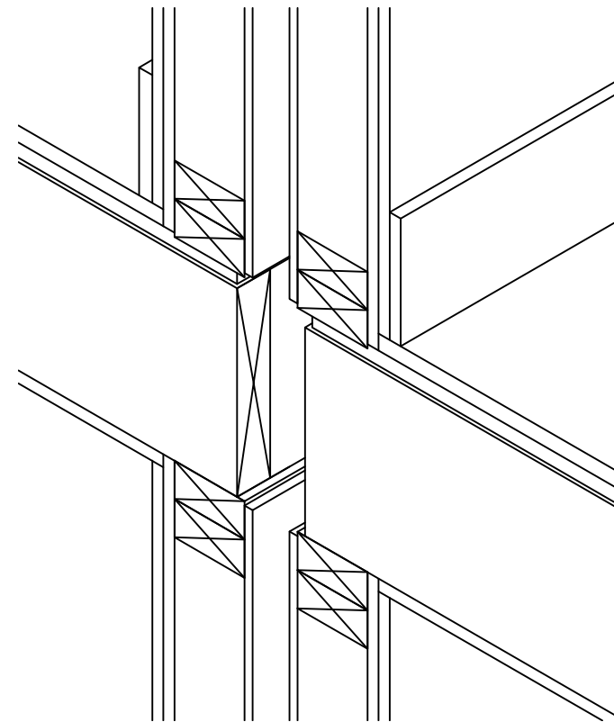
Typical party wall junction
