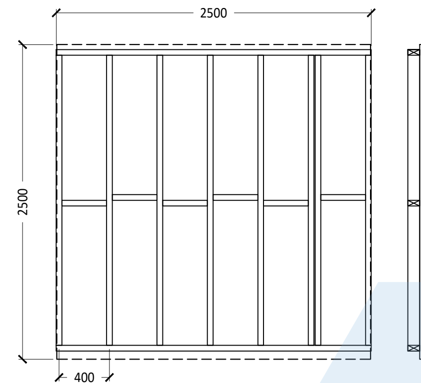
Typical party wall manufacturing drawing
